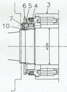
A部詳細 (R:1/2)
