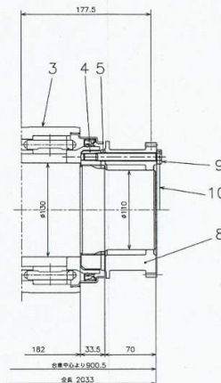
C部詳細 (R:1/2)
